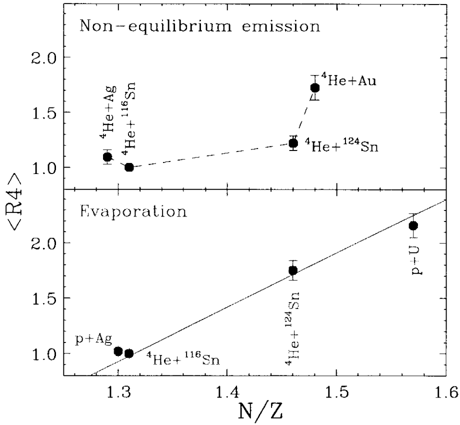
Figure 6: The N/Z dependence of R4 for isotopes produced in evaporation reactions at backward angles (bottom panel) [13,18,19] and for isotopes measured in non-equilibrium emissions at forward angles (top panel) [13, 21].
