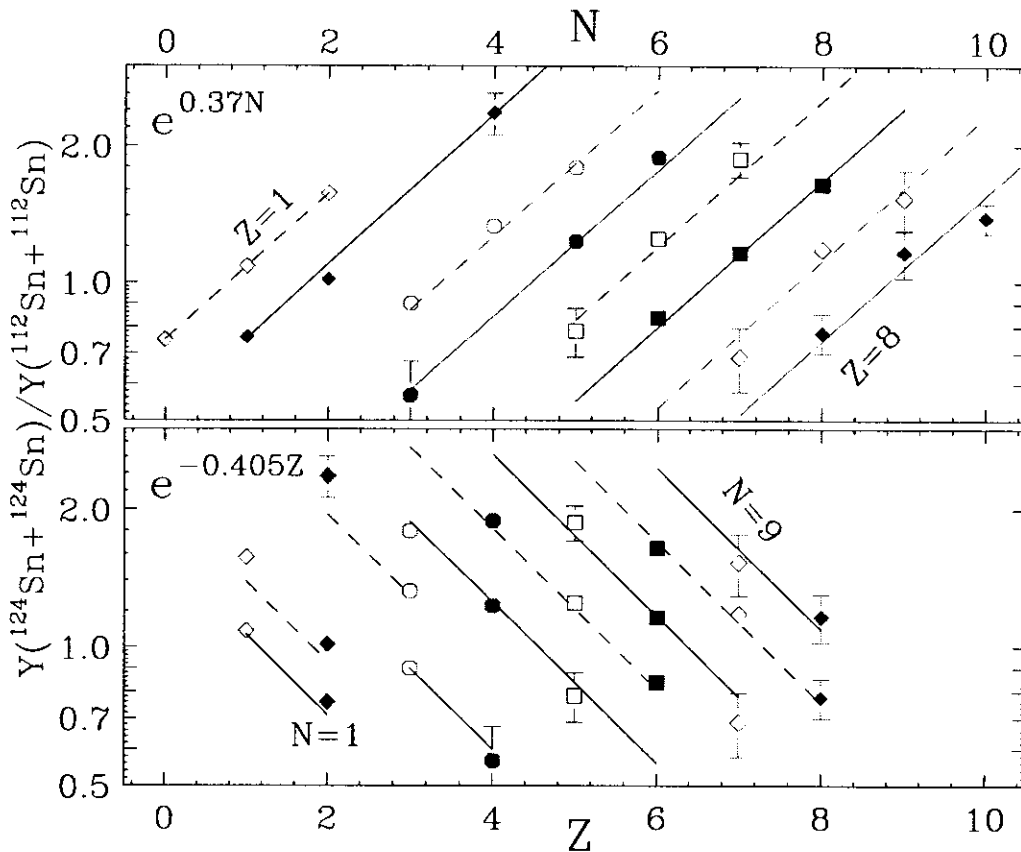
Figure 3: R_{21} for ^{124}\text{Sn} + ^{124}\text{Sn} and ^{112}\text{Sn} + ^{112}\text{Sn} systems, as a function of N (isotope data, upper panel) and as a function of Z (isotone data, lower panel). Solid and dashed lines are best fits to the data.
