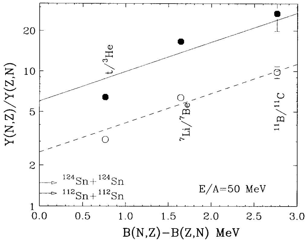
Figure 2: Isobar ratios for three pairs of mirror nuclei obtained from the {}^{112}\text{Sn}+{}^{112}\text{Sn} (open circles) and {}^{124}\text{Sn}+{}^{124}\text{Sn} (solid points) reactions. The lines are best-fit parameterizations of Eq. (2)
