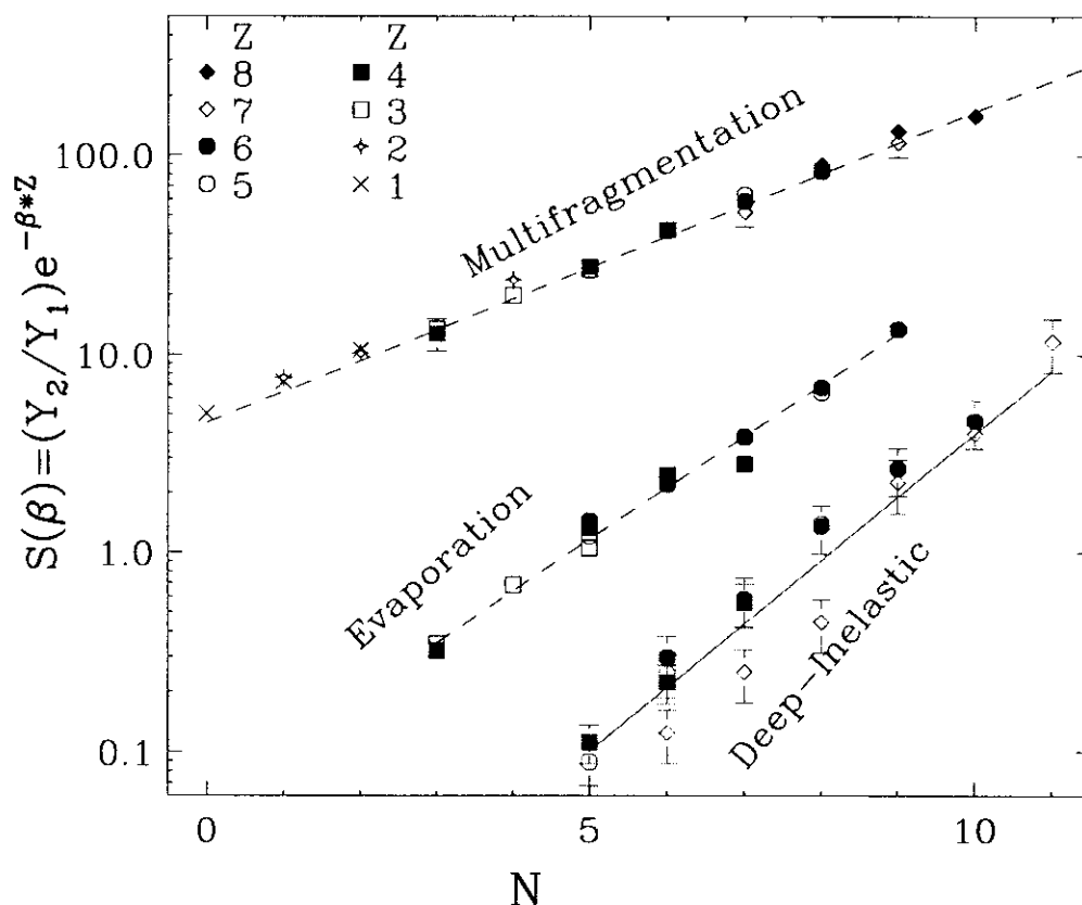
Figure 5: The scaled isotopic ratio, S(\beta) is plotted as a function of N using the best fit value of \beta obtained from fitting isotopes with Z \geq 3 . The data points plotted next to the label "multifragmentation" denote S(\beta) extracted from multifragmentation events in proton density, assuming the same total matter density for the two systems, iscentral ^{112}\text{Sn}+^{112}\text{Sn} and ^{124}\text{Sn}+^{124}\text{Sn} collisions [5]. The scaling behavior for evaporation process is illustrated by the reactions ^4\text{He}+^{116}\text{Sn} and ^4\text{He}+^{124}\text{Sn} [13] plotted next to the label "evaporation". Systematics of the strongly damped binary collisions is represented by the data of ^{16}\text{O} induced reactions on two targets ^{232}\text{Th} and ^{197}\text{Au} [14] plotted next to the label "deep-inelastic".
